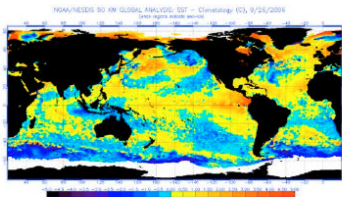
Figure 2. Example of the emerging El Niño for 2006.
