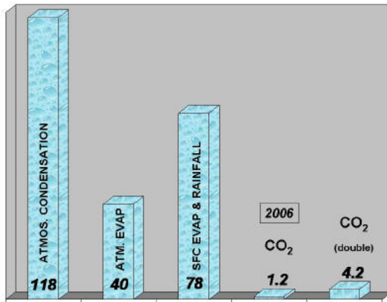
Figure 7. A comparison of moist energy sources and sinks (in \text{Watts}/\text{m}^2 ) of condensation-evaporation-rainfall in comparison with the energy gains due to CO 2 since the industrial revolution ( \sim 1.2 \text{ Watts}/\text{m}^2 ) and for a doubling of CO 2 by the late 21 st century.
