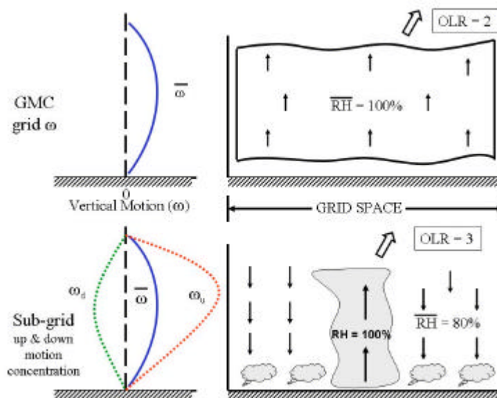
Figure 11. Idealized portrayal of how the grid size of the GCMs is too large to accommodate the real sub-grid scale vertical motion. GCMs can't resolve (top) the concentrated rain or the surrounding cloud downdrafts and subsidence within the scale of its grid space (bottom). The top and bottom diagrams contrast the mean vertical motion of the GCM (top) and the real up-and-down vertical motion of nature. Note that the unresolved vertical motion of the top diagram allows less OLR to escape to space.
