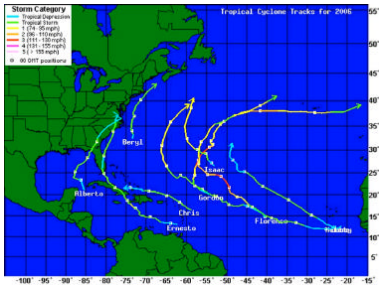
Figure 1. 2006 Atlantic basin hurricane tracks through September 2006.
